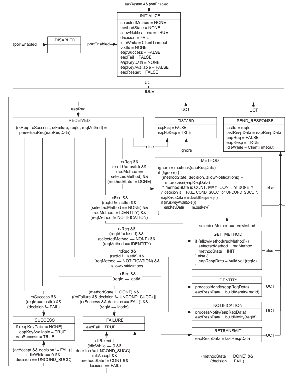
Figure 3: EAP Peer State Machine
