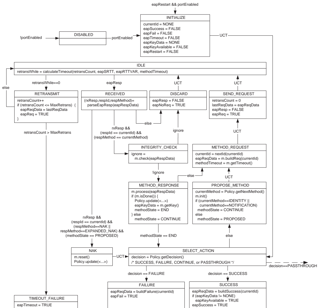
Figure 6: EAP Full Authenticator State Machine (Part 1)
