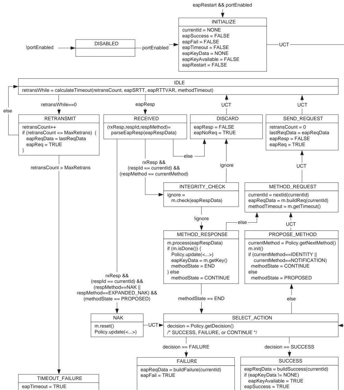
Figure 4: EAP Standalone Authenticator State Machine
