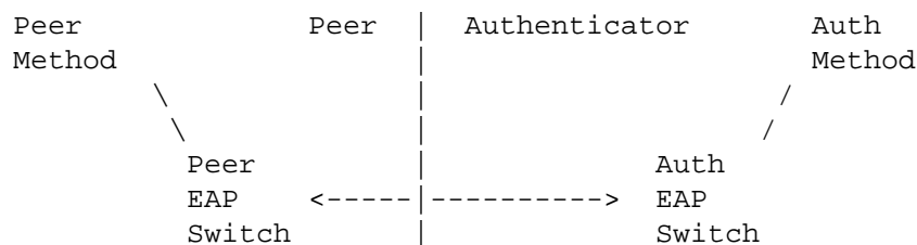
Figure 1: EAP Switch Model
