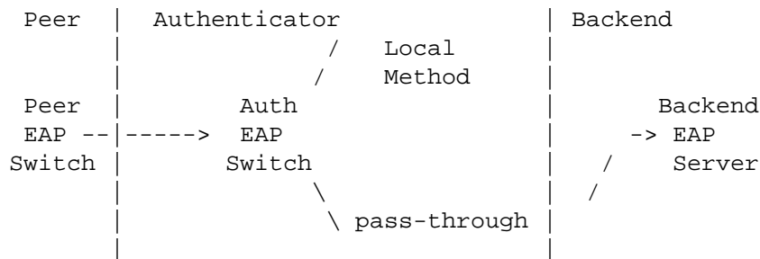
Figure 2: EAP Pass-Through Model
